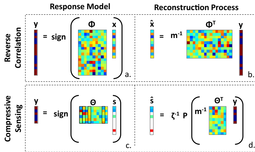
Fig. 2 Process of reconstruction in reverse correlation and compressive sensing. (A) In reverse correlation, the vector of subject responses is modeled as resulting from the multiplication of a latent representation vector ( x ) and a stimulus matrix ( \Phi ), where each row of \Phi is a presented stimulus. This can be thought of as a similarity calculation between the latent representation and a vector representation of each presented stimulus. (B) An estimate of the latent representation ( \hat{x} ) is then reconstructed by regressing responses against the stimuli. (C) In compressive sensing, the vector of subject responses is modeled as resulting from the multiplication of a sparse latent representation vector ( s ) and a compressive sensing matrix ( \Theta ). The compressive sensing matrix is formed by multiplying a matrix of basis
