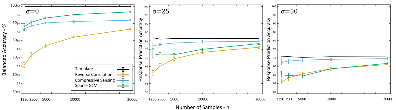
Fig. 5 Response prediction accuracy as a function of sample size. Accuracies (mean and 95% CI) in predicting responses using reconstructions obtained from the template, reverse correlation, compressive sensing, and the sparse GLM from (Mineault et al., 2009) in our stimulation study shown across a range of sample sizes. Estimation quality is shown separately for various levels of noise in the subject
